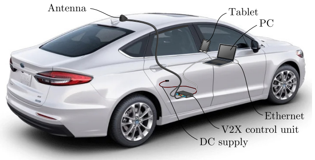
Fig. 2. Vehicle equipped with V2X communication device connected to an upper level computer for data collection and traffic prediction.
